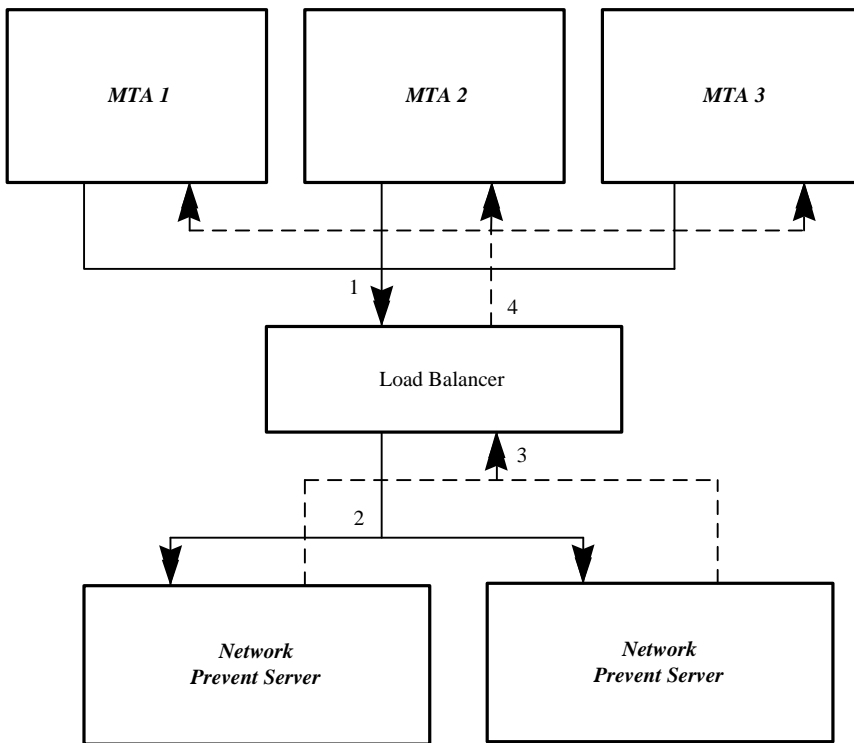
Figure 8: Load balancing with Network Prevent for Email Servers in forwarding mode
