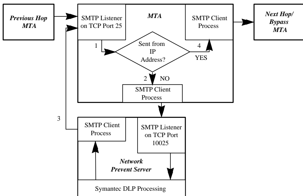
Figure 4: SMTP client IP address-based routing
