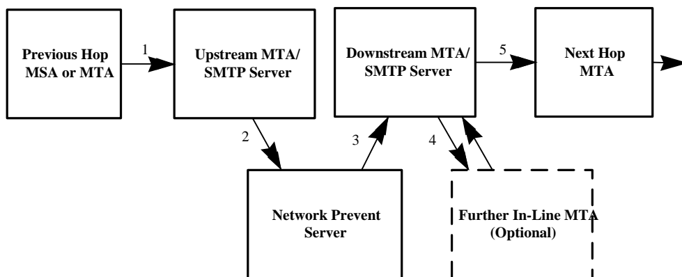
Figure 2: Network Prevent for Email Server operating in forwarding mode
