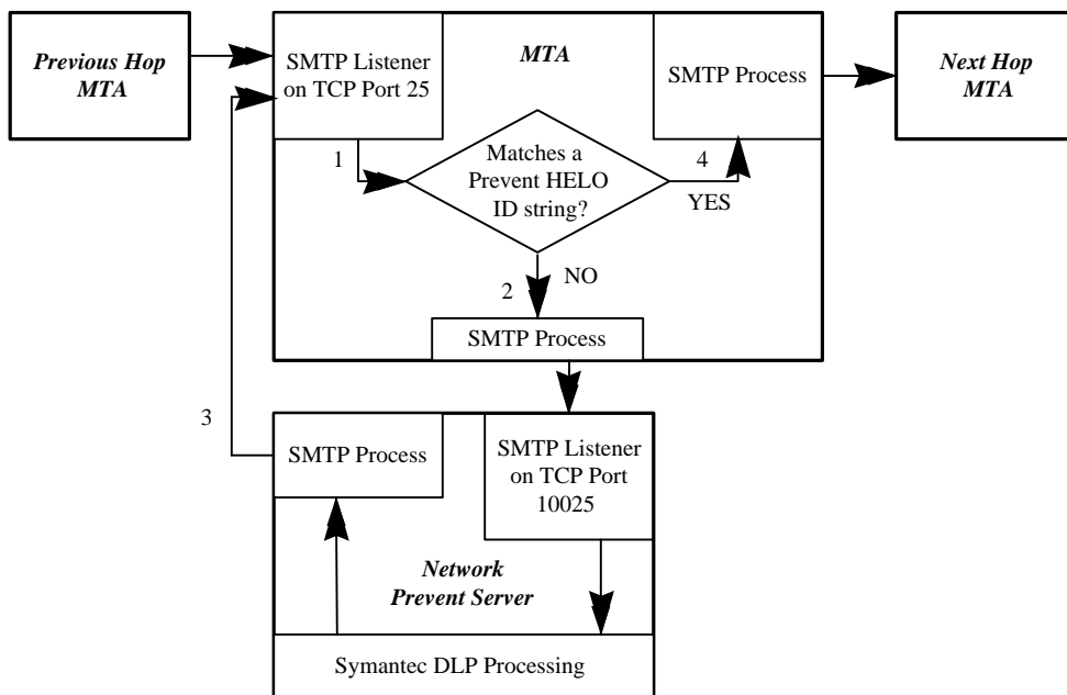
Figure 5: HELO identification string-based routing
