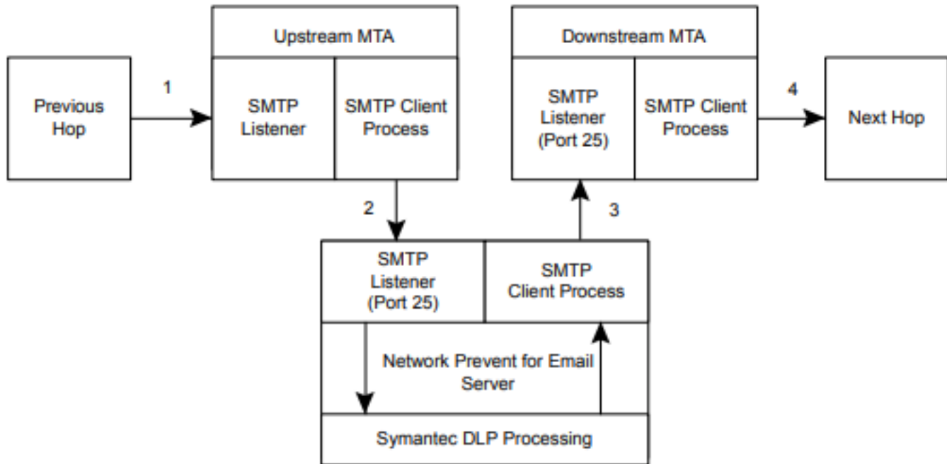
Figure 7: Architecture of Network Prevent for Email Server operating in forwarding mode
