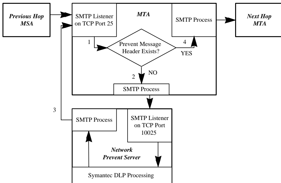
Figure 6: Message header-based routing
